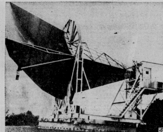
END OF MOONBEAM CIRCUIT —This is the horn reflector receiving antenna used at the Bell Telephone Laboratories hilltop station at Holmdel, N. J., to receive signals during a two-way 480,000-mile conversation between New Jersey and California via the moon. It was the first public demonstration of the principle in the Bell Telephone plan calling for 50 space satellites around the earth to provide quick worldwide communications. (A. P. Wirephoto)
