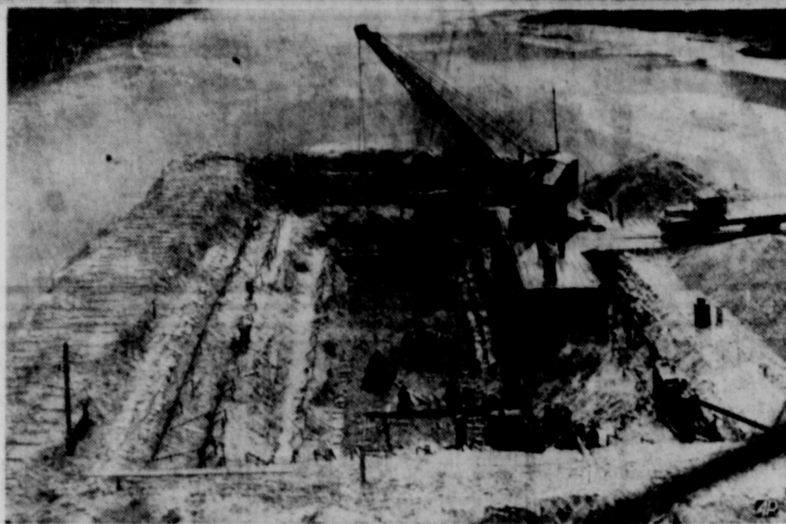
DRY HOLE—Workmen are digging a dry hole in the middle of the Brazos River at Waco, Tex. They plan to set concrete piers in the hole to support the four-lane roadway of a 900-foot bridge. The bridge will extend Waco Drive across the Brazos. V-shaped well-points in the photo pump water from the hole as it seeps in through the sand. (P) Photo
