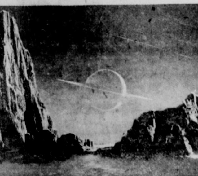
SATURN—with rings, seen from its satellite Titan.
