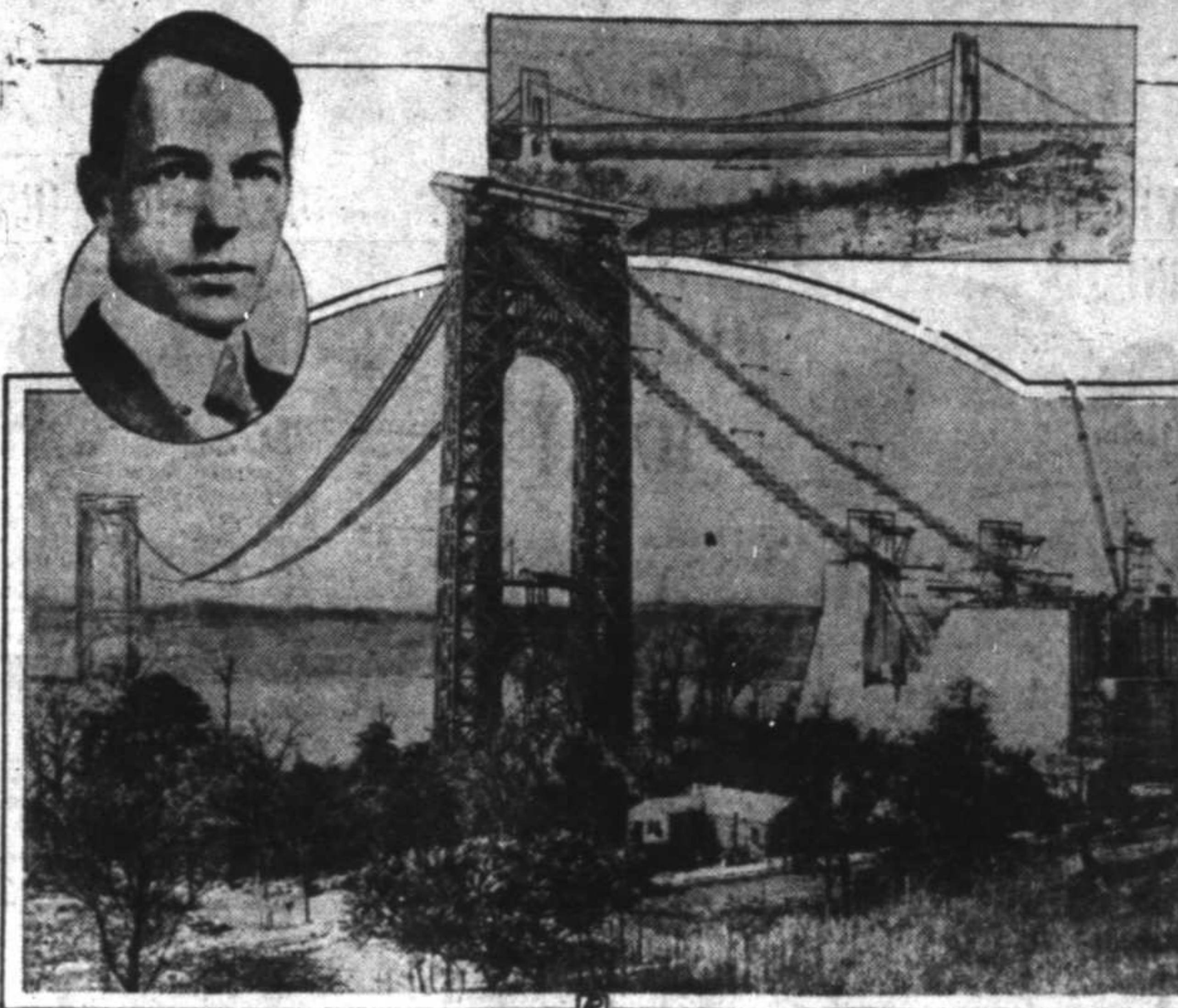
Sweeping two-thirds of a mile across the Hudson river, the world's largest suspension bridge (below) now is half finished. Its towers rise 635 feet on each bank. Architect's drawing (above) pictures completed project, of which O. H. Ammann (upper left) is chief engineer.
