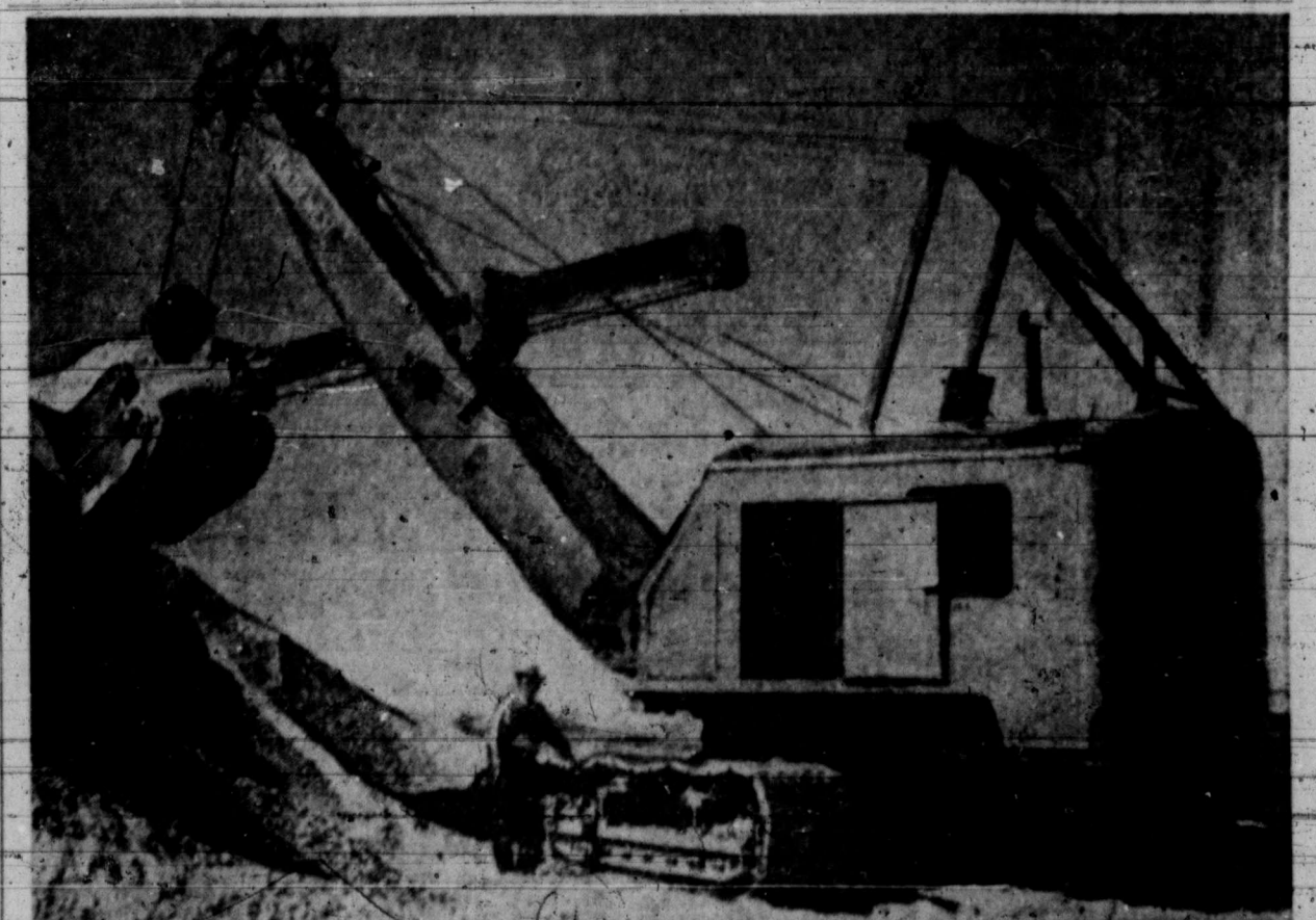
GIANT SHOVEL —Not the kind ordinarily used in spading gardens, but one of the largest to be used on a highway job. The shovel weighs about 73 tons and cost $73,000. Ben Wilkinson, resident engineer for Texas Highway Department, stands beside to illustrate size of the shovel. (Record Staff Photo)
