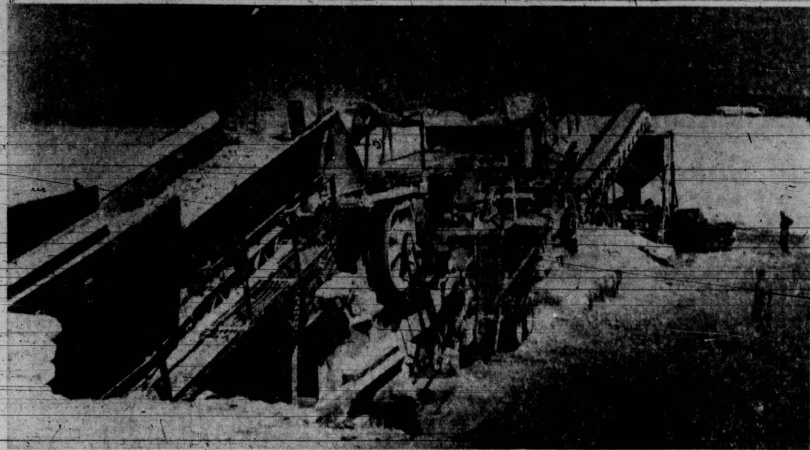
ROCK CRUSHER —This heavy rock crusher being used by Cage Brothers Construction Company is geared for crushing 3000-cubic yards daily. About 273,000 yards will be required for the freeway project west of Colorado City. Caliche will be used for flexible base. The crusher, located eight miles south of Westbrook on the Conway ranch has been in operation ten days and crushed 30,000 yards. (Record Staff Photo)
