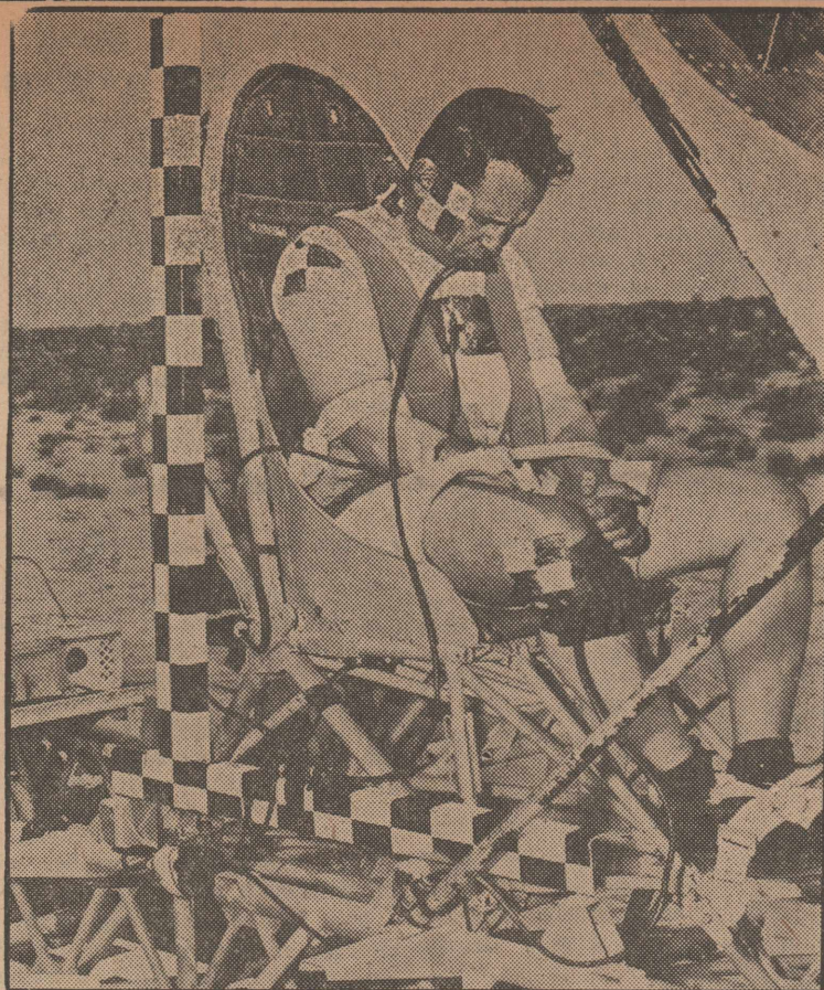
SCIENTIFIC SLED RIDE —Seated on a rocket-propelled "decelerator" sled, Maj. John P. Stapp is ready for a test run at Edwards Air Force Base, Edwards, Calif. Accelerometers attached to mouthpiece, chest and right knee, as shown in this Air Force photo, transmit signals to determine how much impact a pilot wearing safety harness could stand in a plane crash and survive. For his part in many such tests, Major Stapp, a flight surgeon, received the Air Force award of the National Air Council.
