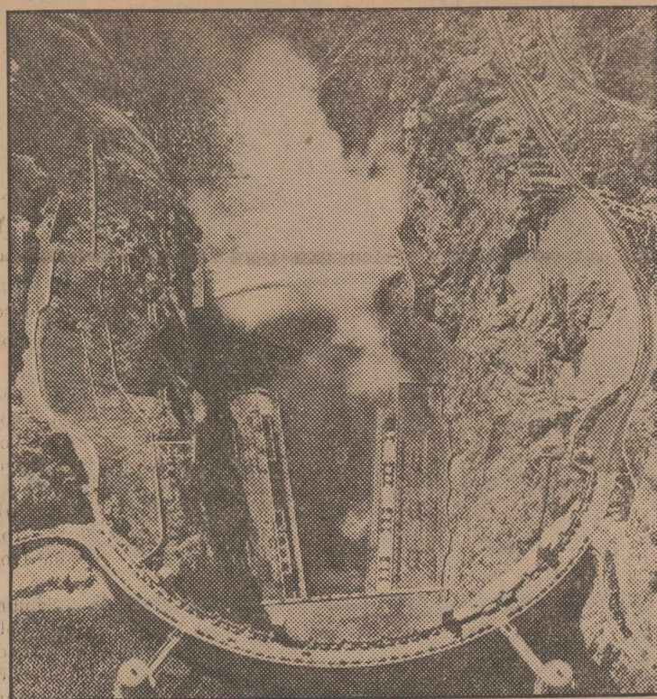
Those slivers of water darting from the walls of Colorado river canyon are actually torrents gushing at rate of 30,000,000 gallons a minute. Scene is Boulder Dam, when emergency outlets were given test. Note cars parked on top of dam and on surrounding roads.
