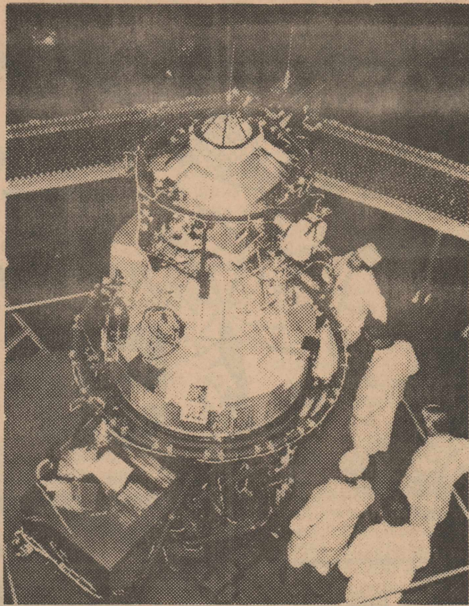
FLIGHT MODEL of the first Earth Resources Technology Satellite (ERTS) is readied for a thermal-vacuum test deep inside a space simulation chamber. The NASA satellite, constructed at the General Electric Space Division, Valley Forge, Pa., is scheduled for mid-1972 launching to inventory earth's natural resources.
