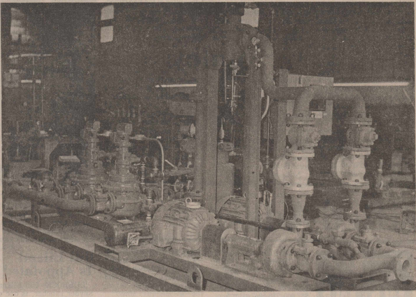
LACT UNIT This LACT unit (Lease Automatic Custody Transfer) has just been fabricated in the I&R shop. Located at 2507 25th St., I&R can custom fabricate just about any piece of equipment needed in the oil patch. (SDN Staff Photo)
