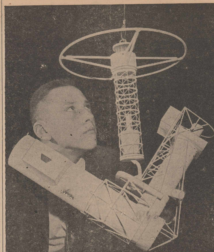
CLEAR VIEW —Visitors at New York's Hayden Planetarium get a good look at the future Stratoscope, shown here one-twelfth its actual size. The Stratoscope is a balloon-borne telescopic camera that is expected to make the first sharp photographs of the planets and other celestial objects.
