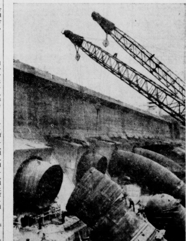
A TRUE PIPE DREAM—Contrasted with the small figures of the workmen, the size of the pipes being fitted into place at the Chief Joseph Dam, in Bridgeport, Wash., is gigantic. The huge steel sections are eased into place in one of the world's greatest hydro-power projects. The dam, on the Columbia River, is expected to start producing power in September, 1955.
