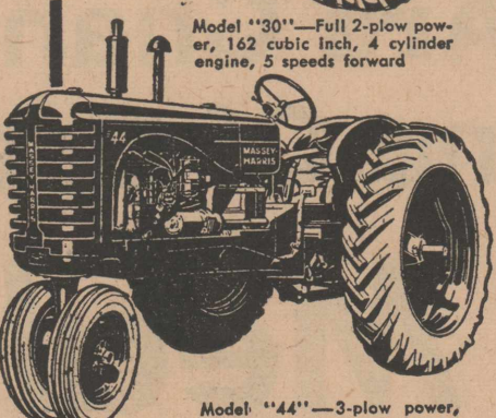
Model "44"—3-pow power, 260 cubic inch, 4 cylinder engine, 5 speeds forward
