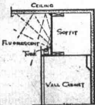
FOR INDIRECT lighting, the soffit is set back from the front of the cabinets, allowing space for concealed fluorescent tubes.
