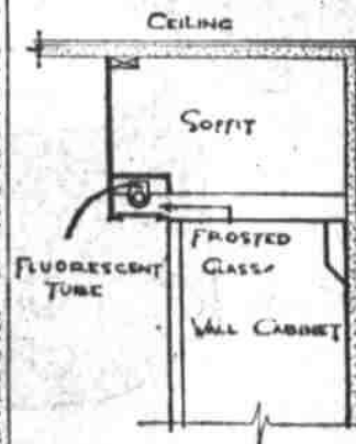
FOR DIRECT lighting the soffit extends over the front of the cabinets with fluorescent tubes above frosted glass panels.
