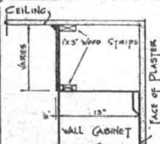
DIAGRAM of a simple soffit formed by wallboard nailed to wood strips on ceiling and cabinet tops.
