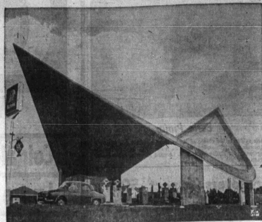
NEW SLANT ON SERVICE —Service station at Retford, England, goes modern with this unusual roof design. Architect calls it a hyperbolic deraboloid structure. It is made of reinforced concrete and weighs about 90 tons. Motel will be added.
