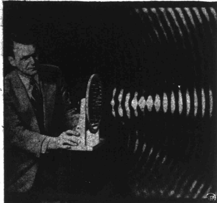
LOOK AT THAT NOISE! — This is an actual photo of sound waves emitted from a horn, taken at Bell Telephone laboratories in New York. The wave pattern, produced during a time exposure of about ten minutes, is made by a scanning technique somewhat like that used in television. A tiny microphone and a 110-volt neon lamp swing vertically through the sound-wave field, producing the pattern which is recorded by an acoustic lens.
