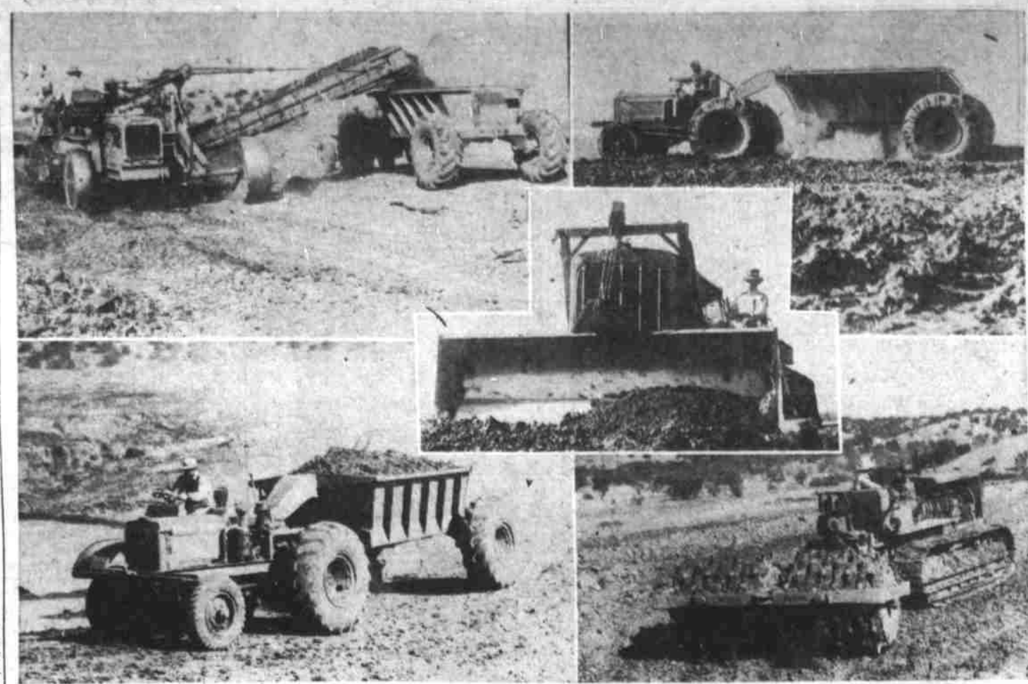
These pictures illustrate how a great volume of dirt—more than 3,500 yards per day—is being moved as work goes on apace at the Powell's Creek dam, unit in the city's new water supply system. UPPER LEFT, a huge elevator scoops up dirt, conveys it to a dump truck, which is filled without the vehicle ever stopping. LOWER LEFT, the big truck zooms up the embankment with its load, and UPPER RIGHT, dumps the dirt on the top. INSET, along comes a big bull-dozer to smooth out the heaps left by the trucks, and LOWER RIGHT, a heavy sheep's foot roller completes the job of packing the dirt after it has been given a thorough wetting. (Photos by Kelsey.)
