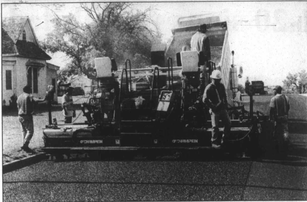
HIGHWAYMEN were using their big "lay-down machine" Tuesday to put a hot-seal mix on Hickory Street as the repaving project neared completion.
