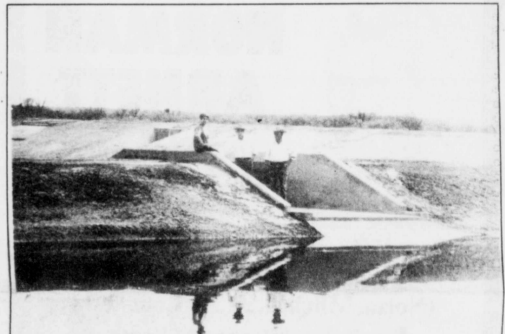
THE HOLDING PONDS on the Morris Hammond property were completed early this week. The ponds are part of the sewer treatment plant project. Pictured are (left to right) Sharon Hammond, Mayor Elmer Martin and Water Works Superintendent Buzz Rich. See related story below.
