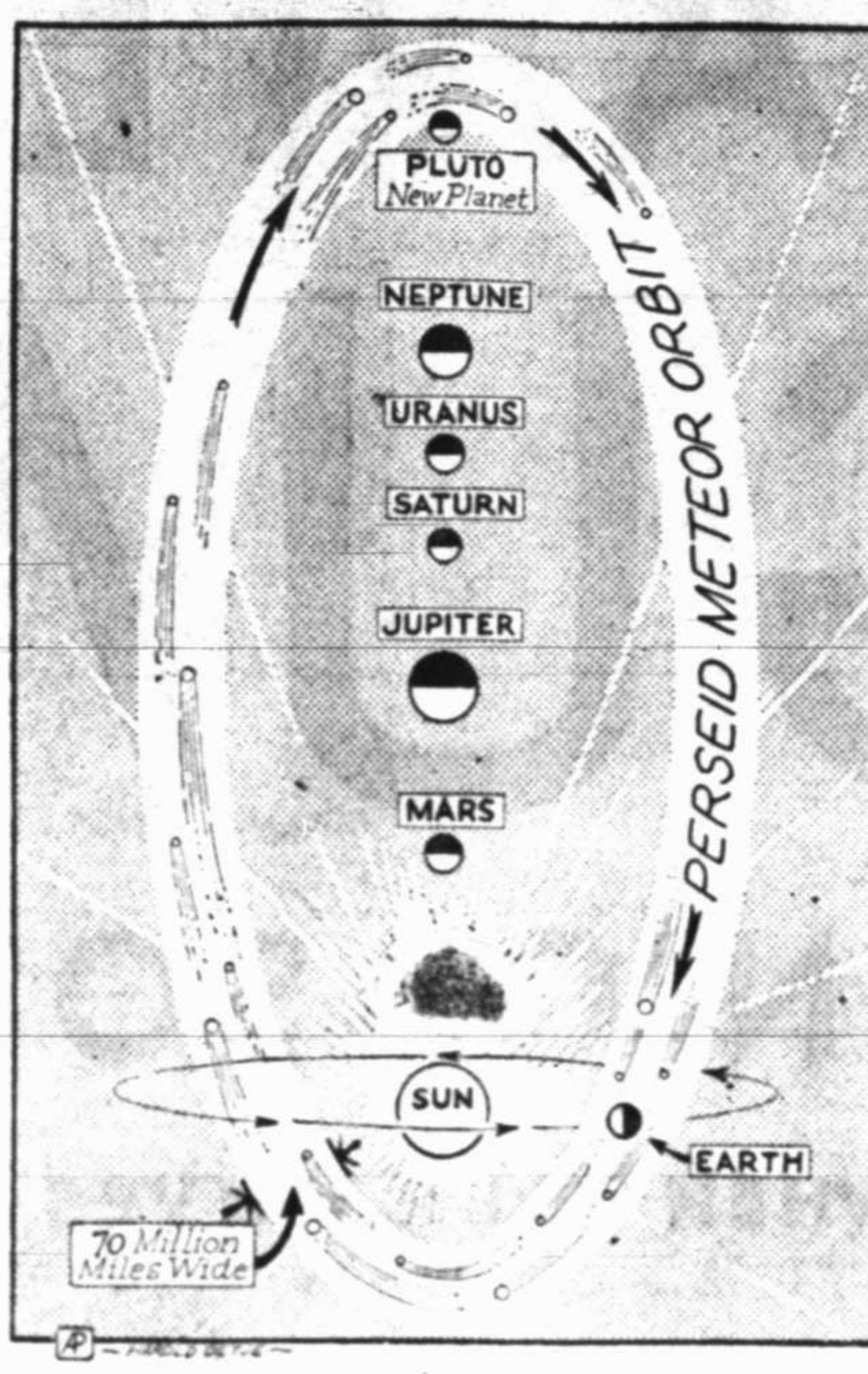
This sketch shows approximate relative positions of principal planets in relation to orbit of Perseid meteors.
