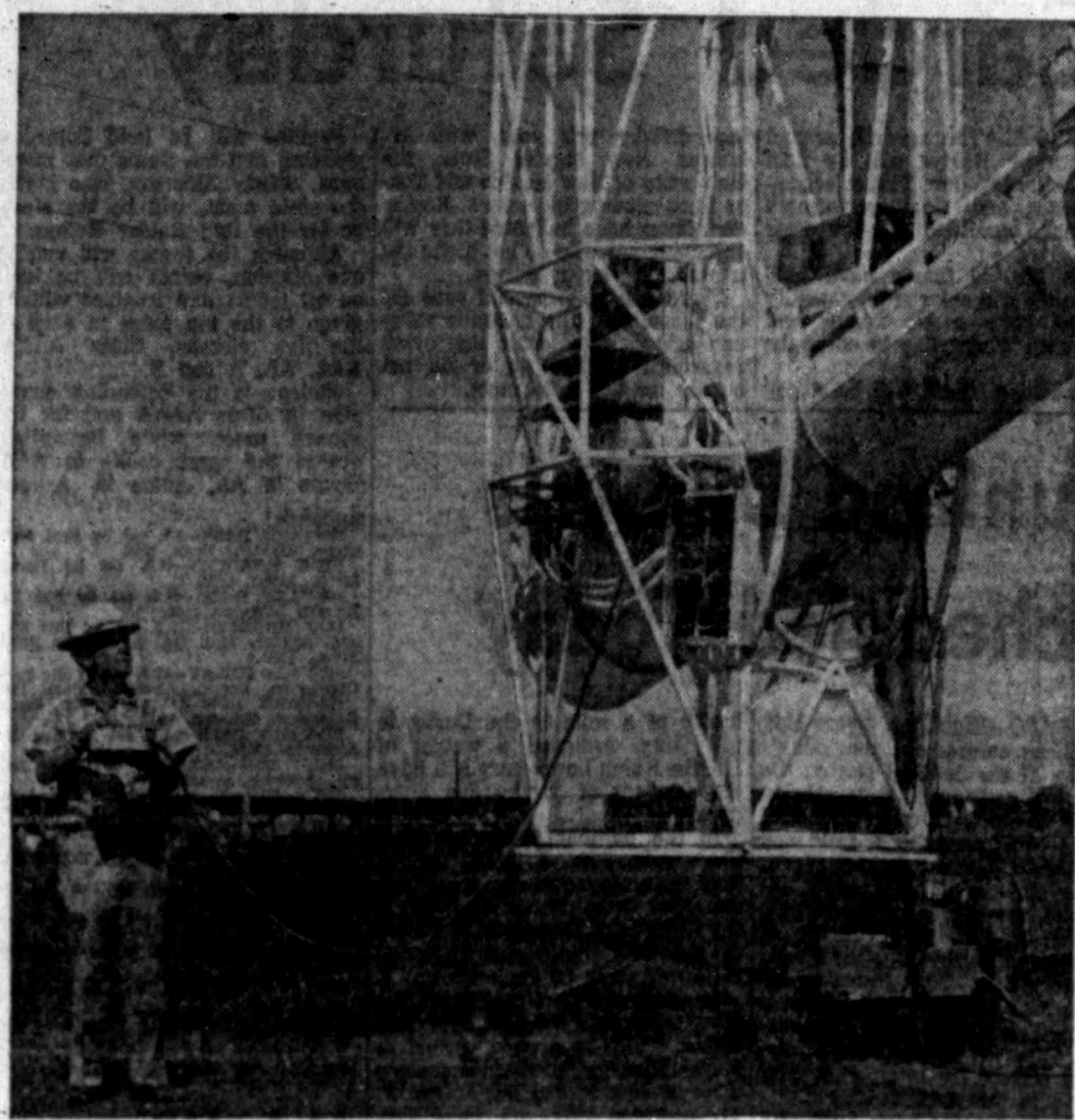
Aerial telescope: Dr. Martin Schwarzschild of Princeton University is shown with the two-ton, 36-inch telescope that will be carried 80,000 feet above the earth to examine the universe unhindered by most of the earth's atmosphere.
