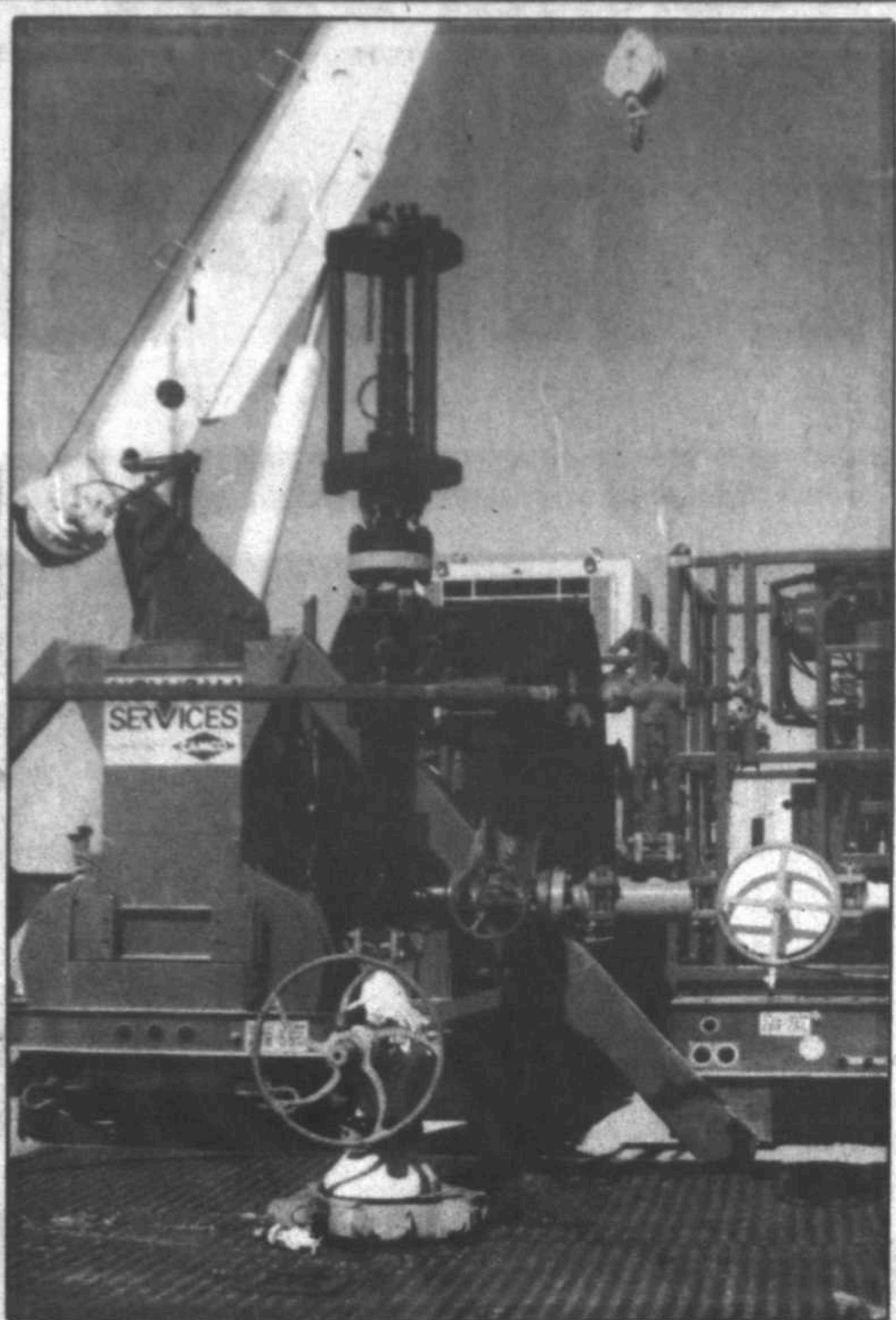
The access window seen on the wellhead above allows for the placement of slips and packoff assembly on a coiled tubing well.
