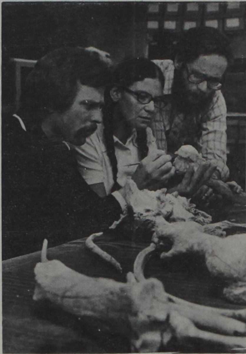
Tule Canyon artifacts
