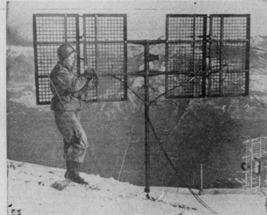
HIGH ON WINDY TOP —PFC L. F. Ferguson repairs UHF antenna atop 6,881-foot Mt. Palon in the Italian Alps near Trento. The station is part of the South European Task Force's vast communications network stretching across northern Italy.
