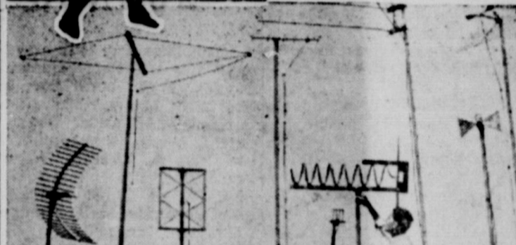
NEW LOOK in television antennas is seen in this display at RCA Victor headquarters at Camden, N.J. These models were developed by RCA engineers to receive telecasts in Ultra High Frequency range which will make possible the opening of more than 2,000 television stations throughout the country.
