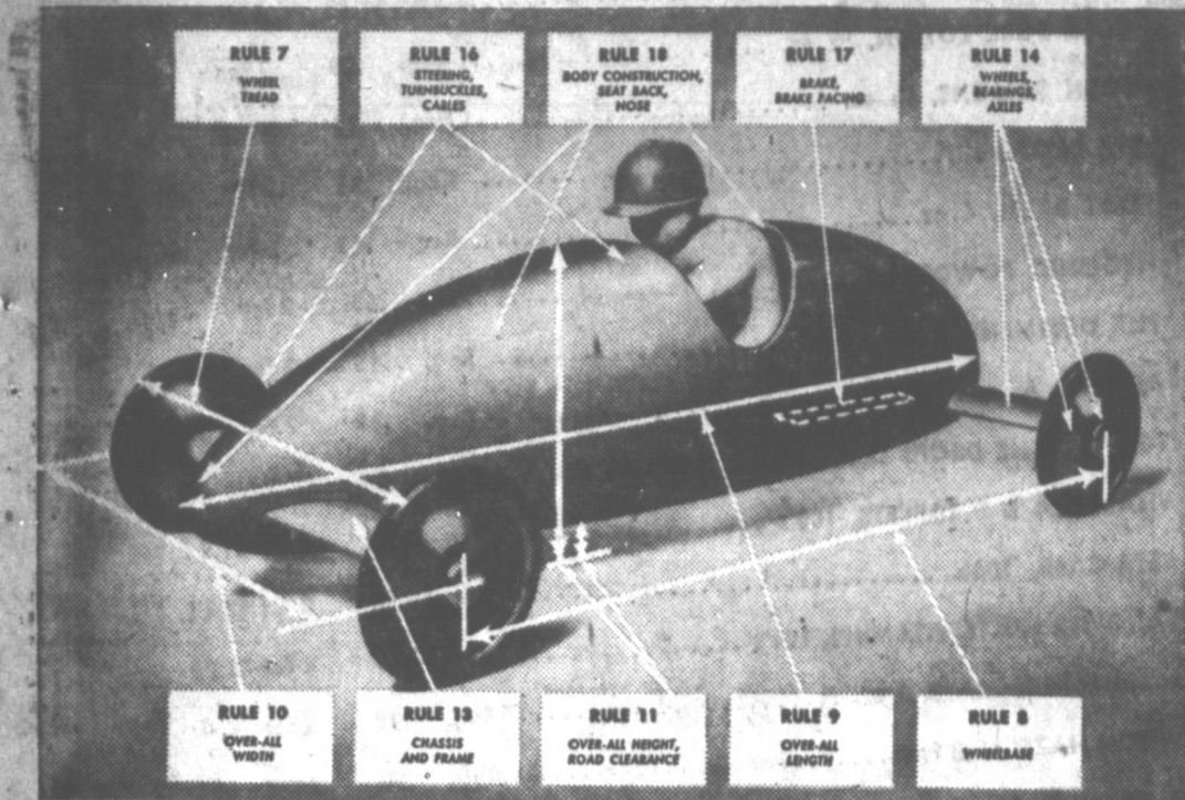
This illustration is a key to the 1949 rule book, showing which section of the book applies to the parts of the car.
