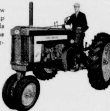
520 SERIES —Full 3-plow power (38-plus h.p.) that ranks up with many larger tractors in work output, with many smaller tractors in first cost and operating economy. Gasoline or LP-Gas engine.
