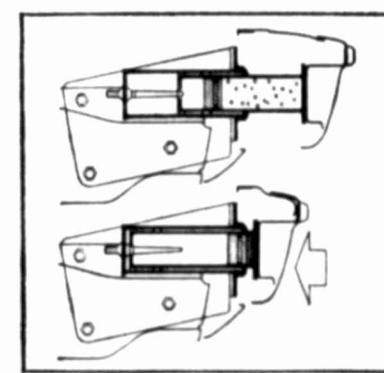
The new energy absorbing bumper system on Hornet telescopes the front bumper as much as 3 inches and returns to normal after repeated 5 mile per hour barrier impacts. It's one of the most advanced systems in the industry.
