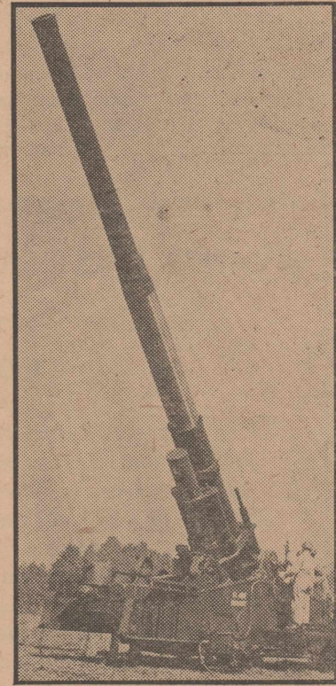
Pointing up 55 degrees, the gun can traverse 360 degrees for effective firing range. Under actual combat conditions the gun would be detached from both transport units.
