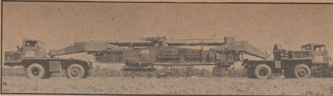
The mobile gun-carrying unit is made up of two six-wheeled cabs and engines, each operating independently of the other. When unit is assembled, the forward cab-engine controls throttle and brakes of both. Total length of gun in transit is 84 feet 2 inches.
