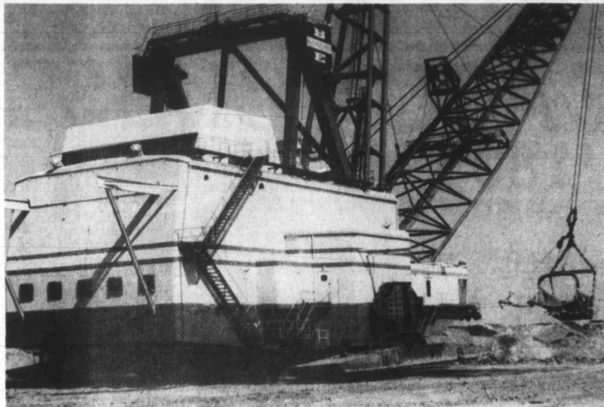
WALKING ALONE — This five million pound dragline is shown walking along as it picks up its platform legs (see lower right side) for one of its nine-foot strides.
