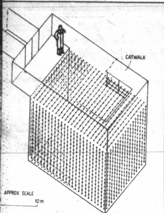
AT'S - EYE view of the IMB proton decay detector. A man is standing on a catwalk that actually surrounds top of the six - story cube. Behind him is the tunnel leading to the detector. The electronic and water filter element has been installed there. Before him, the detector is lined with black plastic and a network of phototubes which are represented by the dots.
