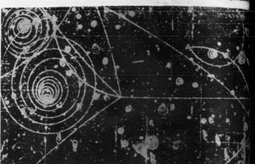
MODERN ART?—In a way, this picture is more modern than any modern art picture to date. It is the type of photograph which led scientists to the discovery of elementary particle of matter, the omega meson. The omega meson, which has an important role in the structure of protons and neutrons—the basic building blocks of atoms—was discovered at the University of California in Berkeley.
