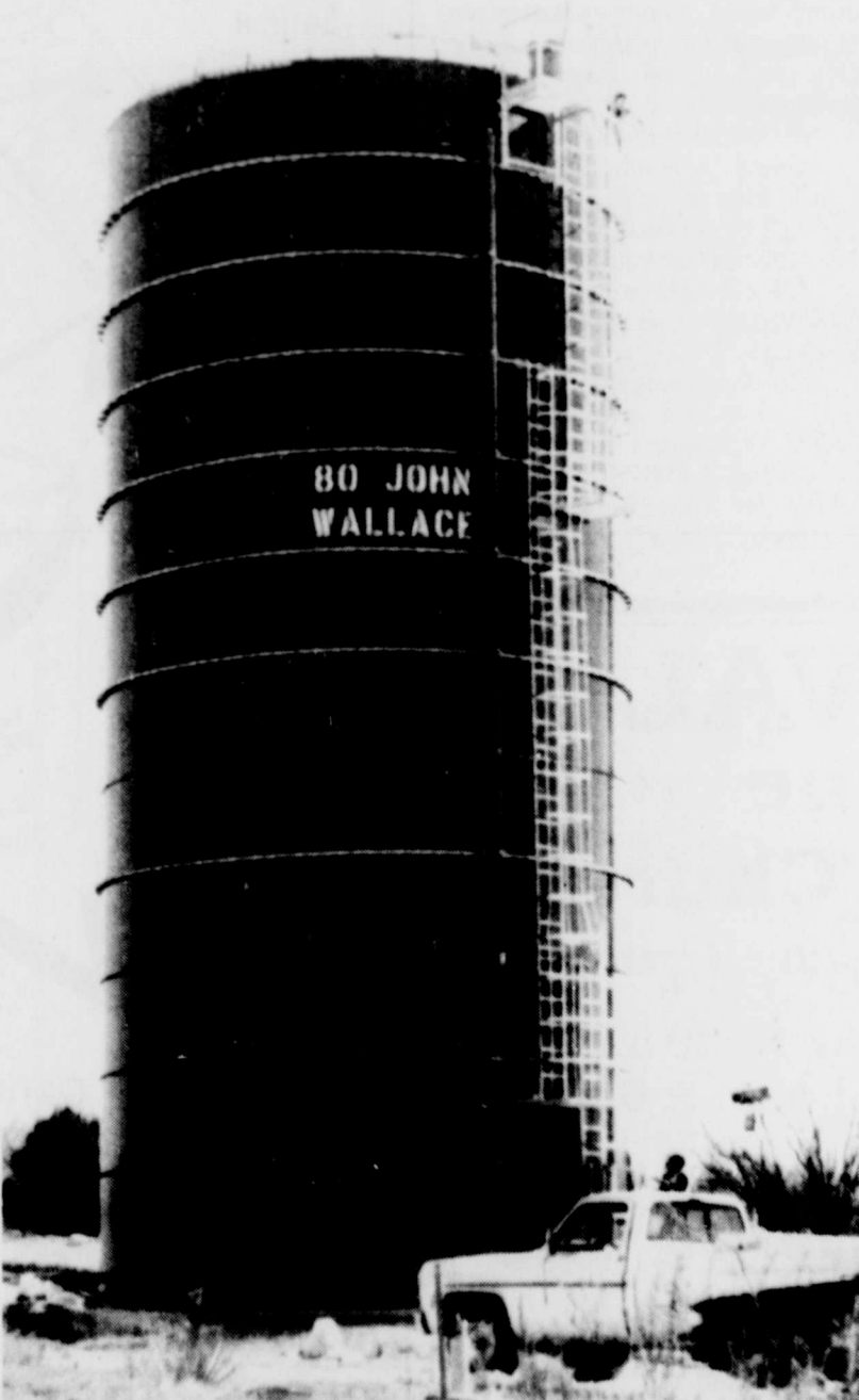
GOING UP IN A HURRY: This standpipe - which will eventually reach 120' in height - is reaching that elevation in a hurry. The tank will hold over 470,000 gallons and will serve primarily the Texas Department of Criminal Justice facilities although it is looped into the city's water system.
