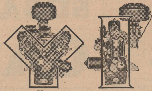
The new V-block V-8 with the new extra-deep crankcase, has 130-h.p. for a dividend of 18% more power. And you can enjoy V-8 advantages on less gas!
