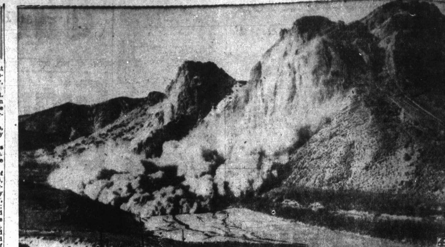
BIG NOISE IN WYOMING — Contractors on the Boysen Dam, Wyoming, needed 150,000 cubic yards of rock fill so they exploded two carloads of TNT in the side of a mountain along the Wind River. The roar could be heard fifty miles away.
