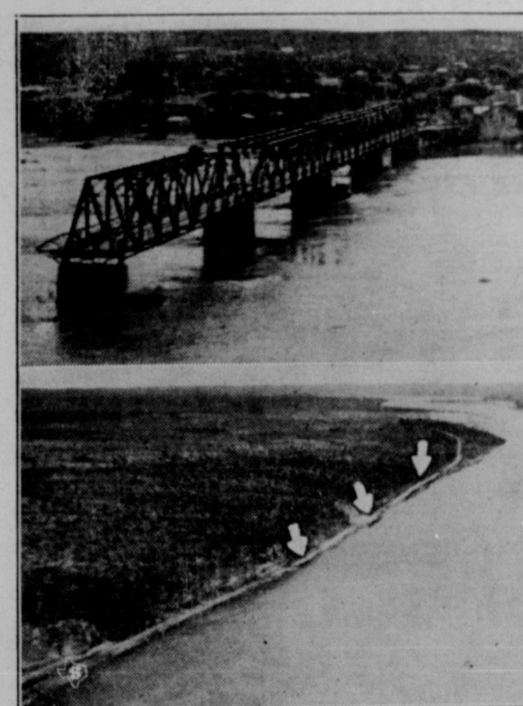
The top photo is a closeup aerial photo of the bridge over the Rio Grande river showing how the middle spans were washed away by debris piling up against them as the muddy waters swept towards the sea. Below is a section of the Southern Pacific tracks near Del Rio, inundated by the Rio Grande.
