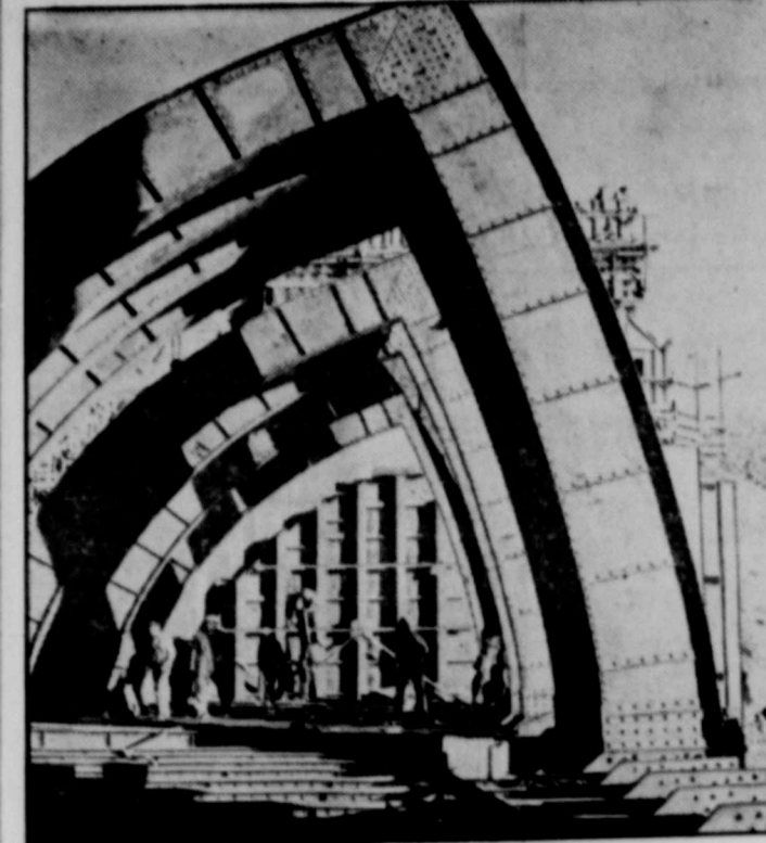
A bit of Gothic art makes its appearance at Grand Coulee Dam in the State of Washington, where this huge drum gate is assembled above a compartment in the spillway crest of the storage reservoir. Eleven of these 135-foot gates, largest ever built, will be used to control the level of water in the dam's reservoir.
