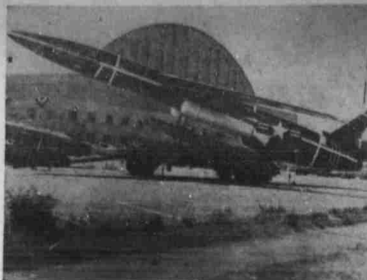
MOBILE LAUNCHER FOR SNARK - Buffalo, N.Y. - The mobile launcher for the U.S. Air Force's Snark, shown here with the 5,000-mile missile in firing position, has been ordered in production quantities for the first time. The launcher, which also serves as the missile's carrier, makes it possible for the Snark to be moved rapidly from place to place and to be fired from any level surface.
