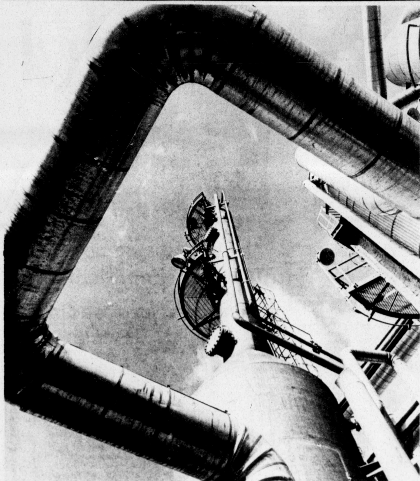
Bird's-eye view is assured from the top of this tower at PPG Industries' ethylene glycol manufacturing plant at Beaumont. The firm also manufac-
