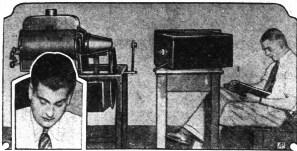
Reception of television signals broadcast from station WIXAY, Lexington, Mass., has been reported from New York State and Connecticut. A projector, whirling disc containing a spiral of 48 holes, and a set of photo electric cells are the essentials of the studio equipment shown above. Alfred J. Pote (lower left), is the engineer in charge.
