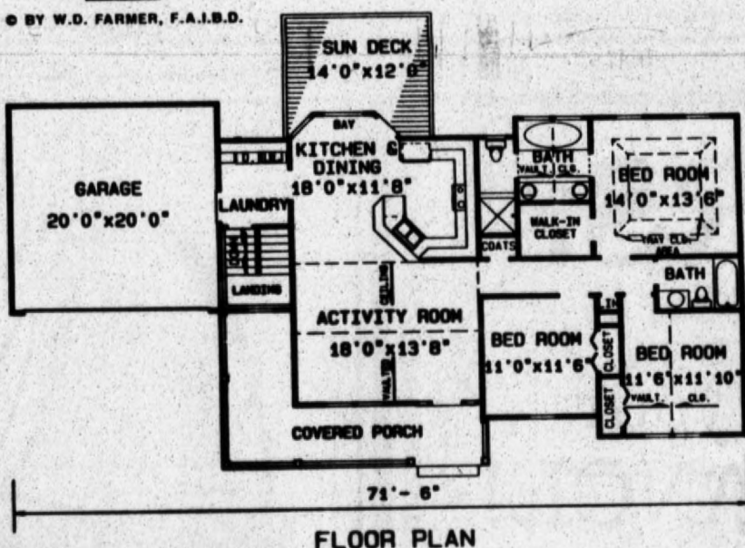
FLOOR PLAN
