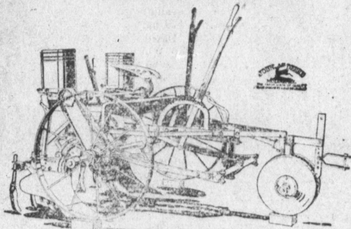
JOHN DEERE NO. 660 TWO-ROW LISTER
