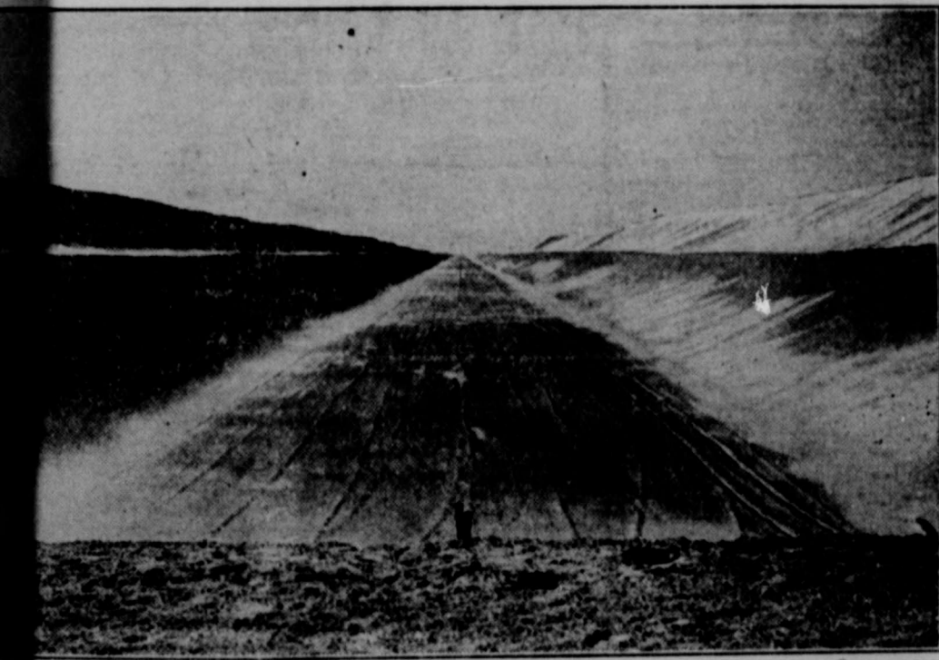
A BIG DESERT DITCH AWAITS ITS FLOW OF WATER New view of the 80-mile-long All-American Canal, built by the Federal Bureau of Reclamation across the desert. It parallels the Mexican border through Southern California and will provide irrigation for hundreds of thousands of acres of arid lands in the Imperial Valley district. For the greater part of its course it is 260 feet wide.
