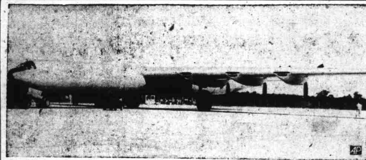
WORLD'S LARGEST LAND-BASED BOMBER—The world's largest land-based bomber, Consolidated-Vultee XB-36, is being readied for its initial ground tests. The bomber is a pusher type aircraft powered by six 3,000 horsepower Pratt & Whitney engines, has a wing spread of 230 feet, and a fuselage length of 163 feet. Initial tests are scheduled for later in the summer, depending on the completion date of ground and taxi tests. This picture was taken June 1 at Fort Worth, Tex. (AP Photo).
