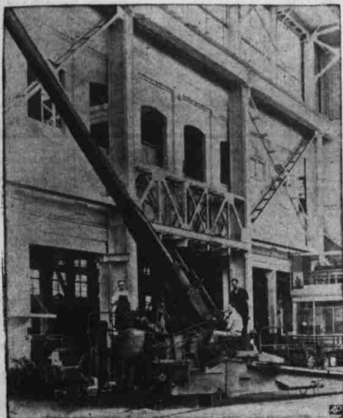
BIG GUN FROM YORK —Two York, Pa., companies collaborated to build this new 8-inch mobile gun for the U. S. Army, shown in final assembly in the S. Morgan Smith plant, normally making hydraulic turbines. The York Corporation, maker of refrigeration and air-conditioning equipment, was the partner. Assembly line ran through both plants.
