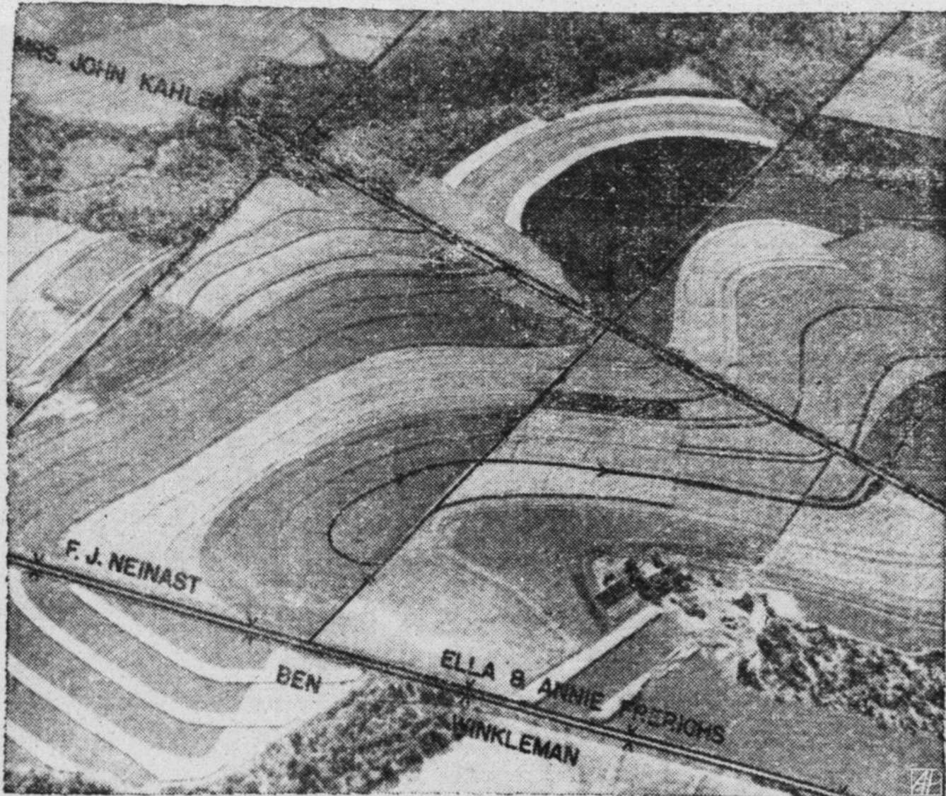
Cooperation has been written on the land in the Elm Creek watershed near Temple. This aerial view shows terrace lines crossing farm boundaries to empty into a grassed drainage channel that crosses two farms and runs into a natural drainage on the farm of Mrs. John Kahler at the foot of the slope. One terrace (arrows), the outlet channel and farm boundaries are marked to illustrate how farmers have cooperated to solve a common problem—soil erosion.
