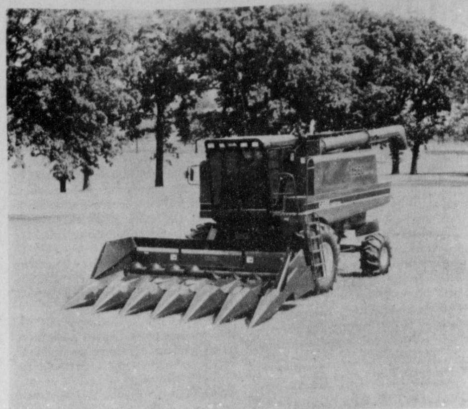
RACINE, WI, September 1985...The new Case International 1600 Series Axial-Flow combines feature higher horsepower, increased elevator capacity and a new feeder and header reverser. The Model 1660 combine, rated at 180 horsepower, is shown with a Model 1063 6-row narrow corn head.
