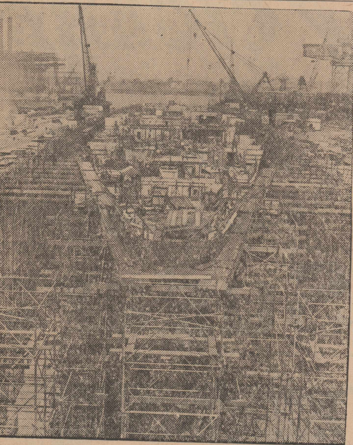
SHE'S A-BUILDING A lacework of scaffolding surrounds the superaircraft carrier USS Saratoga, now under construction at the New York Naval Shipyards, Brooklyn. N. Y. Her keel laid in December, 1952, the Saratoga will be the largest craft of her type in the world when completed about January, 1956.
