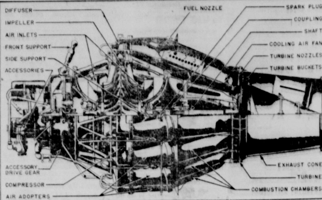
INSIDE A JET ENGINE—More powerful than any reciprocating aircraft engine is this General Electric J-33 design of a jet engine which drives the Lockheed P-80 Army Air Forces fighter, called the "Shooting Star." The engine, which delivers 4,200 pounds of thrust, is shown above.
