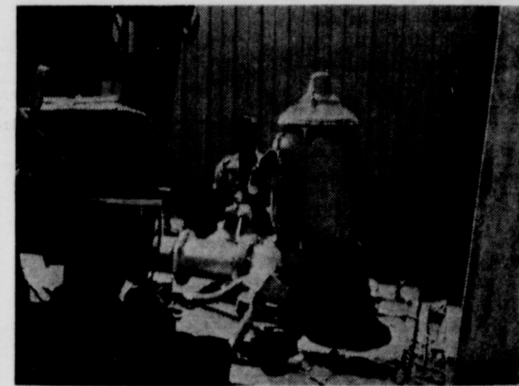
THE WELL RIG, owned by Houston and Joe Dean Smith, shown above, left, had just finished lowering the pump 20 feet in the city water well on Sixth Street. Joe Dean Smith is shown coupling the discharge pipe to the pump. A few minutes later the electric pump motor was turned on, and an interested crowd of men tensed as the motor roared for what seemed like an eternity before muddy water started gushing from the discharge pipe. To the group gathered there, the muddy water looked better than a flowing oil well would have. After the water cleared up, this well was placed back on the city water system to relieve the water situation which had developed Wednesday of last week.
