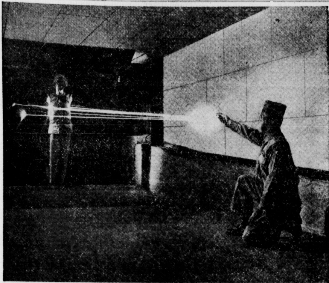
TESTING!—Bullets from the pistol of Lt. Col. Walter R. Walsh, USMC, ricochet harmlessly or imbed themselves in a "shrapnel jacket" during a test of the body armor in Washington, D. C. The new type of protection, now used by troops in Korea, is made of laminated glass cloth and synthetic resin. It has been more than 90 per cent successful in preventing wounds.
