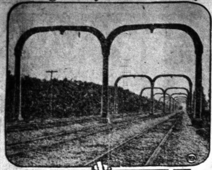
Railway men throughout the country are watching with interest Henry Ford's experiment of electrifying his railroad, the Detroit, Toledo and Ironston. Photo shows a stretch between Dearborn and Flat Rock, Mich., where electrification is complete. The big arches carrying the power wires are made of concrete, cast in two pieces, and Ford has built a special factory to make them. He will install them eventually all along the line.
